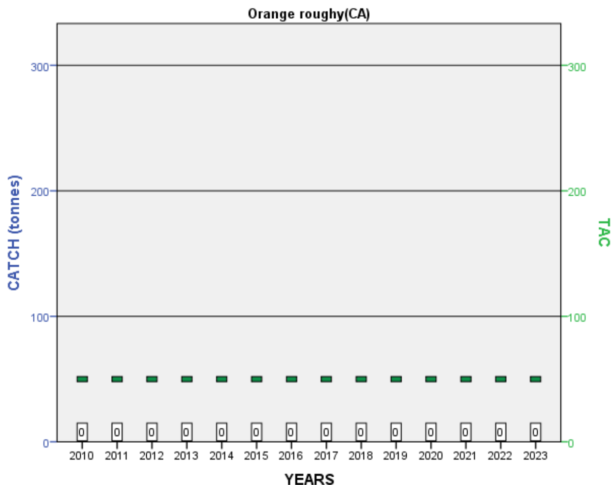
Figure 4: Orange roughy catches and set TAC outside the B1, since 2010.
